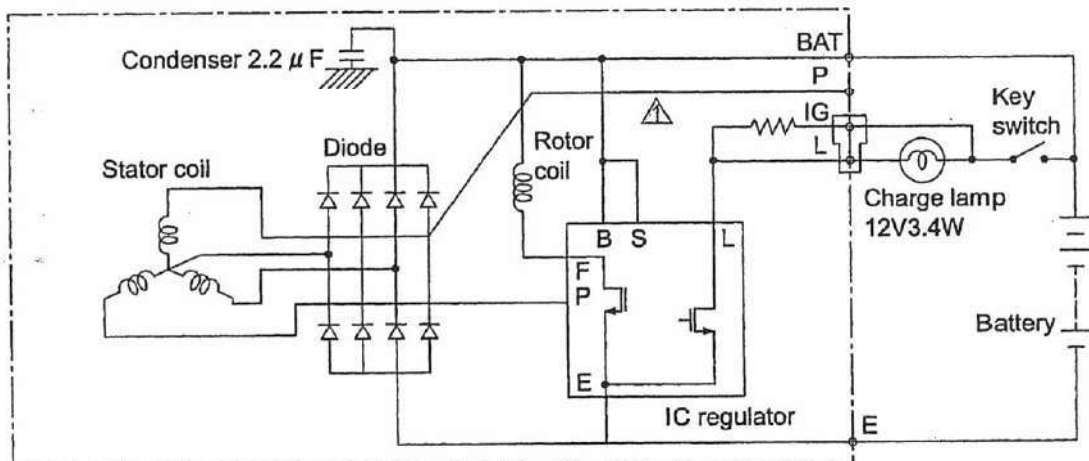
Alternator
