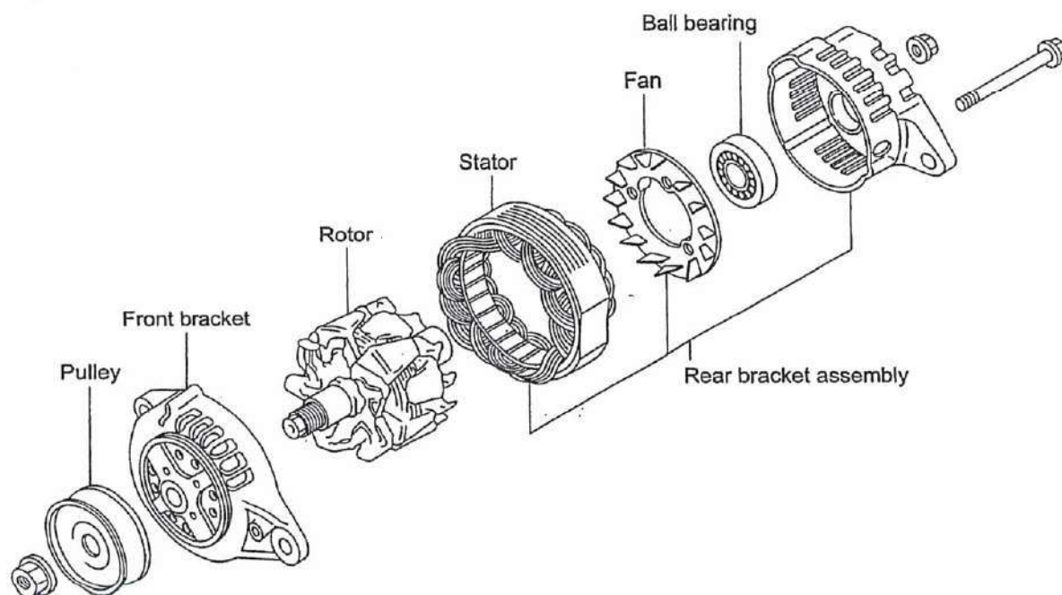
(12V60A alternator)
