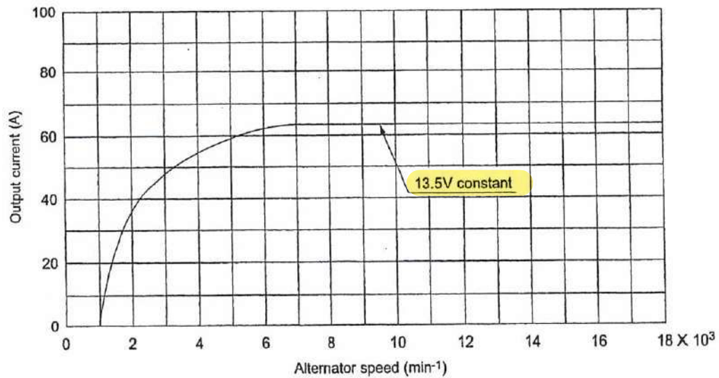
Alternator
