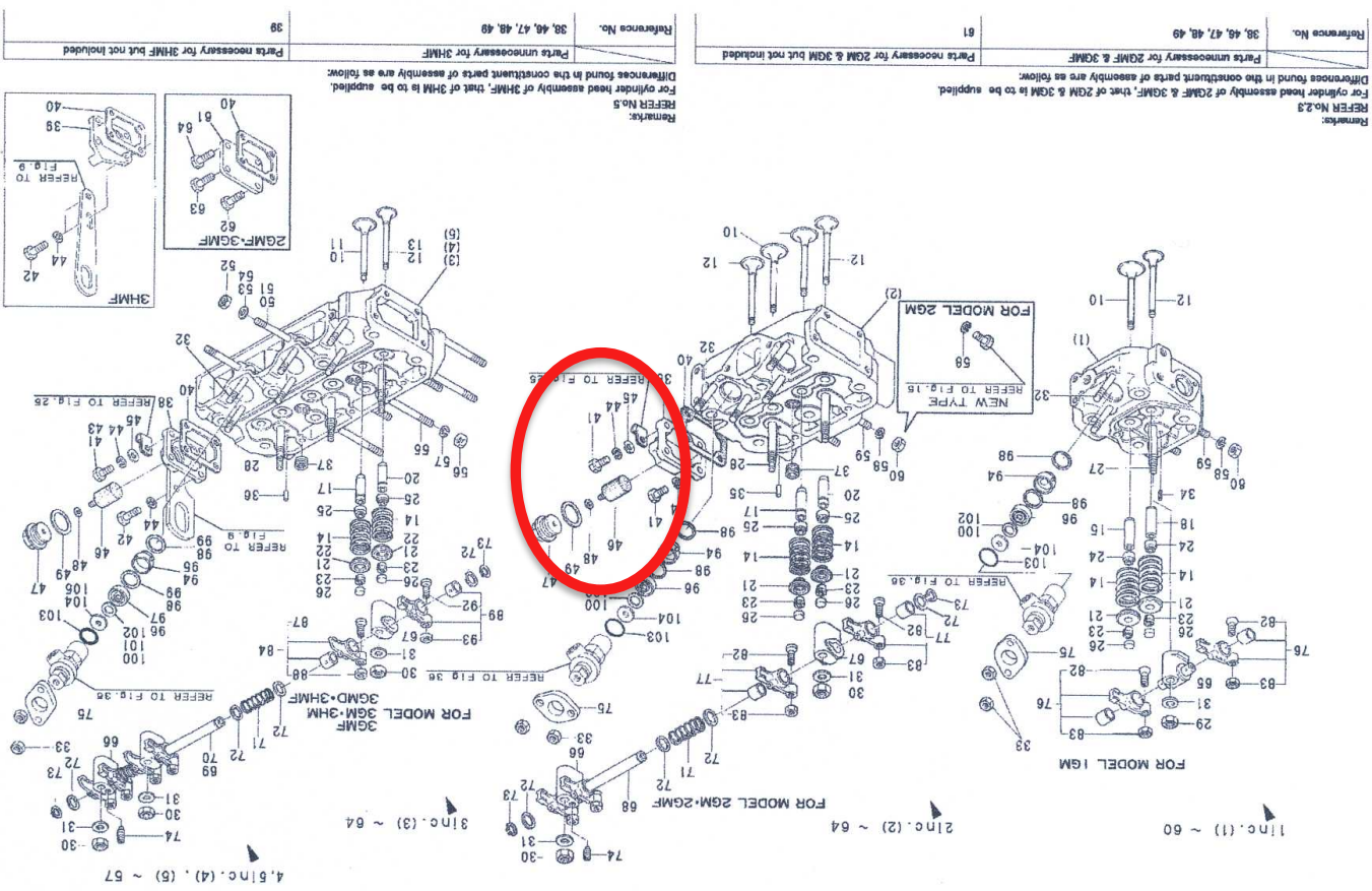
Fig. 11. CYLINDER HEAD
