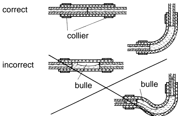
Fig. 805 Raccords tube-tuyau
