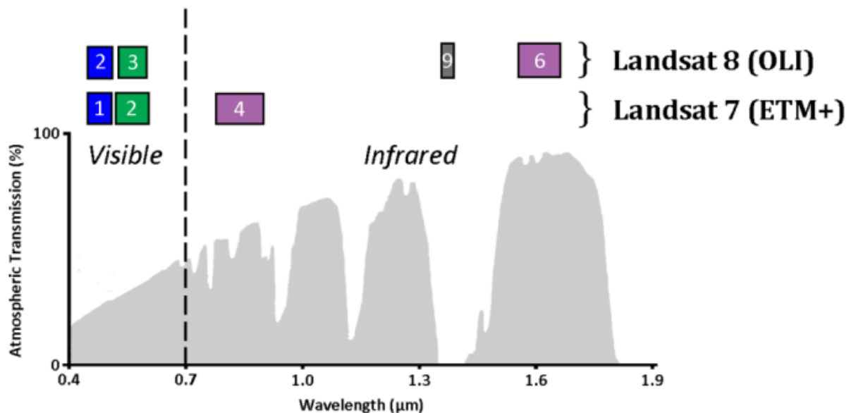
Bands of Landsat 7 and 8 imagery used in the SDB procedure.
